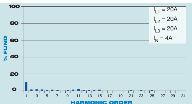
Neutral harmonic current with PQF
