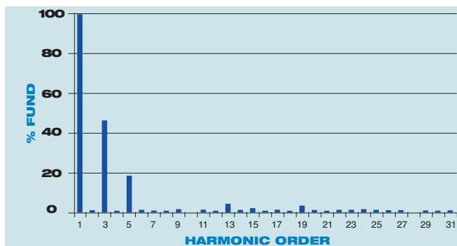
Neutral harmonic current without PQF
